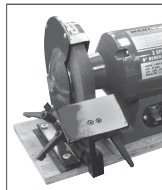
Fig. C - Grinding Platform
