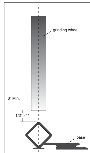
Fig. A - Mounting
