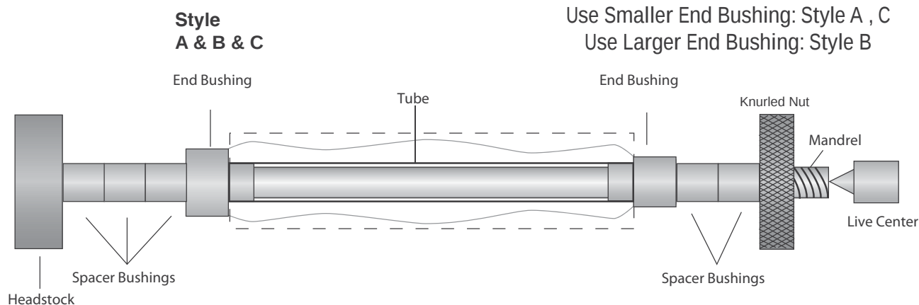
Diagram B - Turning the Blank
