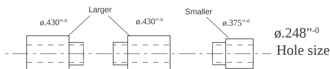
Diagram E - Bushing #PKSRBU
